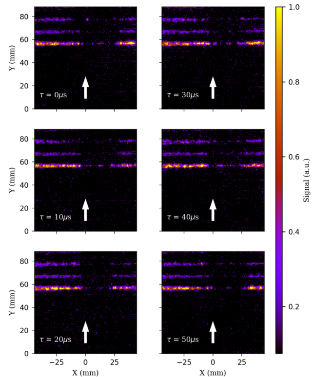
Fig. 6. 6-image sequence of 100-kHz PLEET in the Tunnel 9 freestream measurement of Mach 18.
