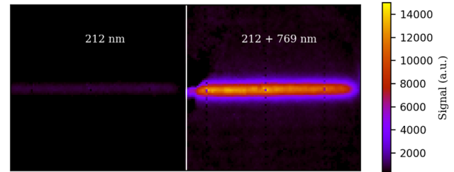
Fig. 2. Comparison of the “read” beam effect in a static cell with 10-torr pure Kr. The result shows that the “read” beam has 10\times signal enhancement for a delay time range of 100–300 ns.
