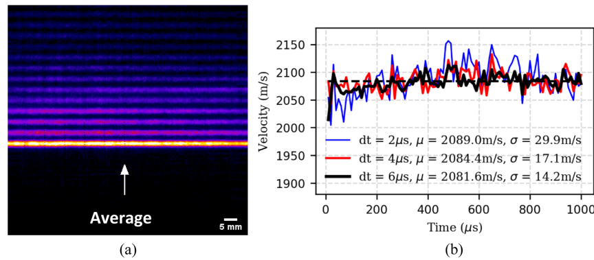
Fig. 5. (a) Average 100-kHz KTV image and (b) a time series of the flow velocities measured by a single burst in the AEDC tunnel 9. The dashed line in (b) is the mean velocity.
