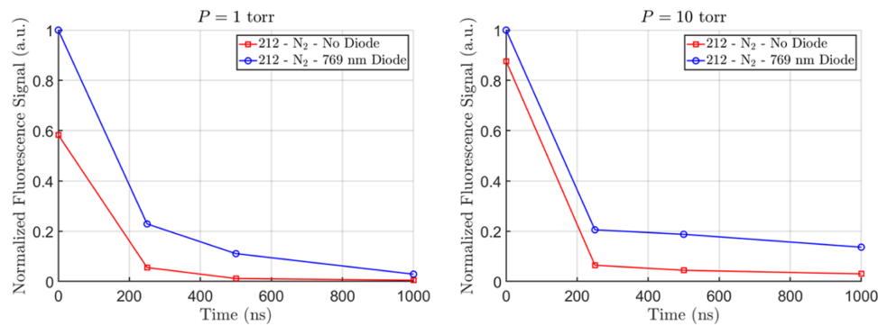
Fig. 3. Time-resolved comparison of the “read” beam effect in a static cell with 99% N_2 /1% Kr at pressures of 1 and 10 torr. The “read” beam enhances the 212-nm excitation signal by a factor of 4–10, depending on the delay time.
