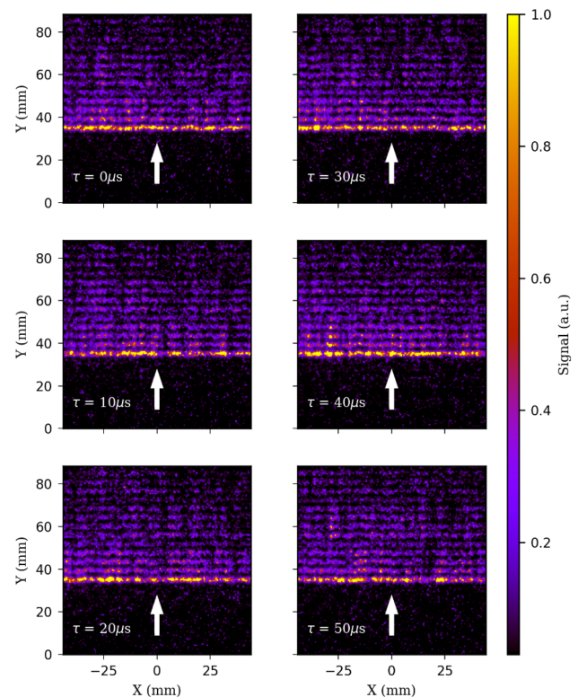
Fig. 4. 6-image sequence of 100-kHz KTV in the Tunnel 9 freestream measurement of Mach 18.
